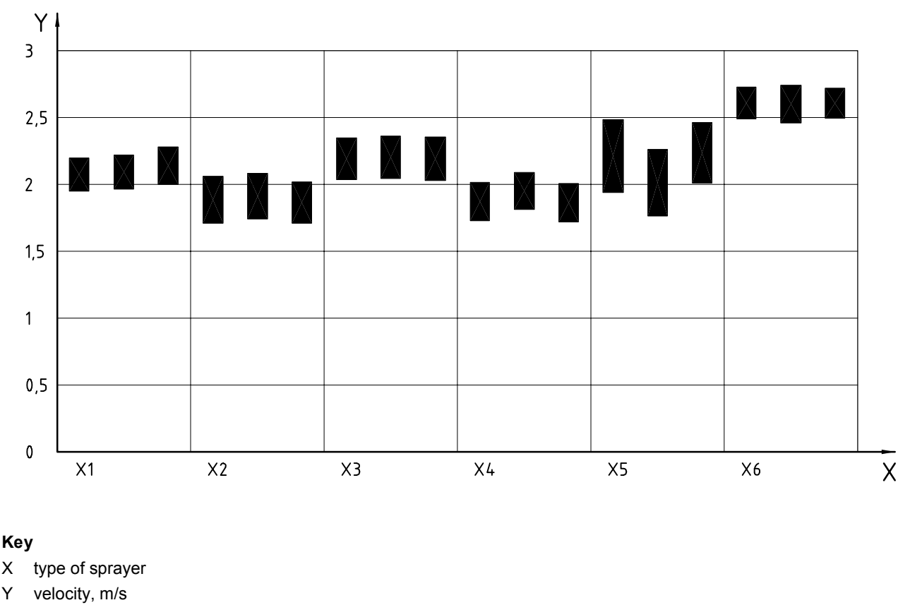
Figure D.2 — Standard deviation of spray boom movements in horizontal plane (deviation against average velocity of spray boom) — Three repetitions
